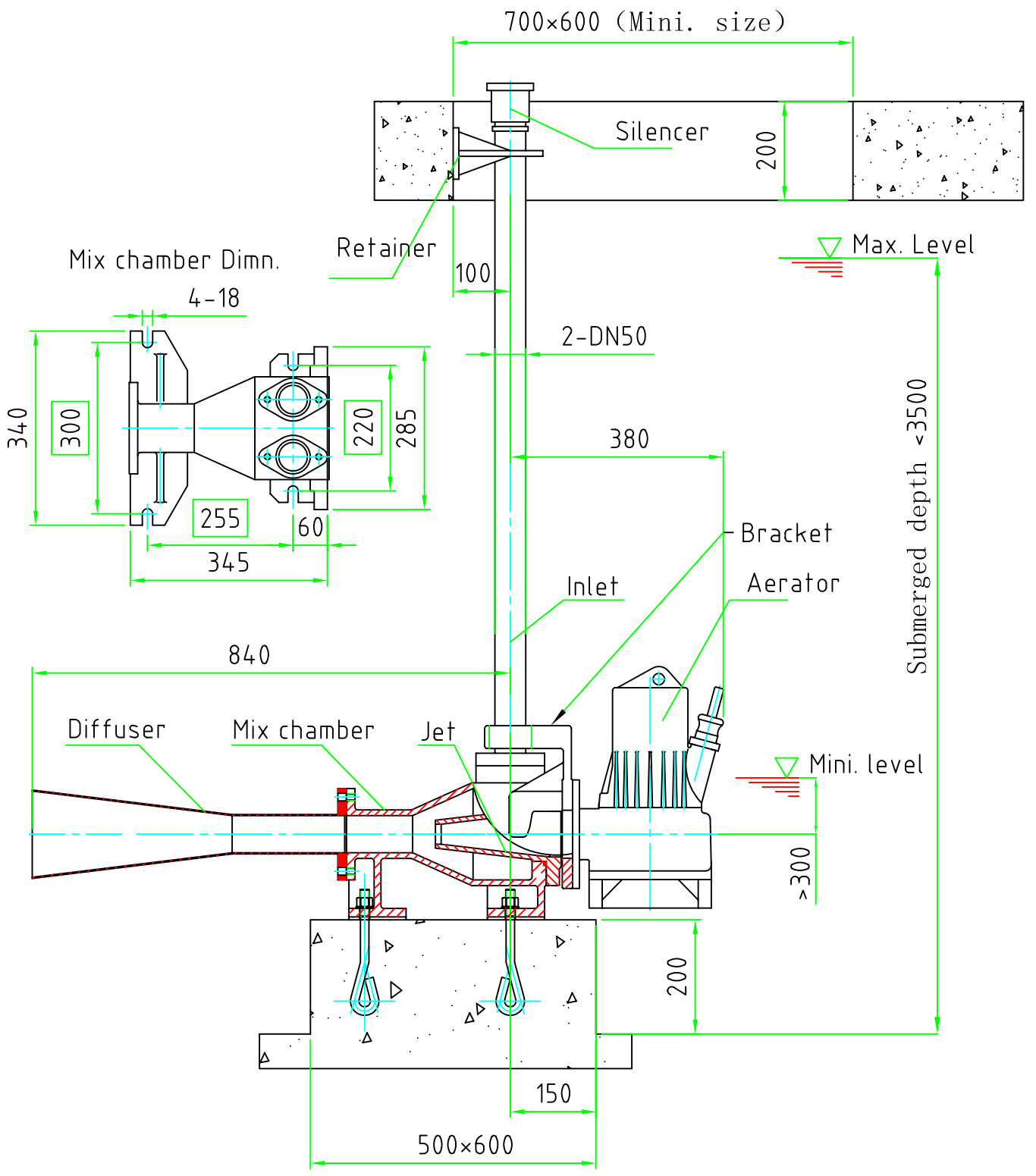
QSP0.75 Dimn.
